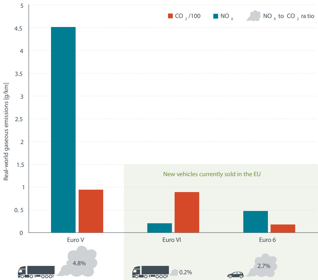
Figure 3. Average real world NO x and CO 2 emissions of Euro V/VI/6 heavy-duty and light-duty vehicles.
